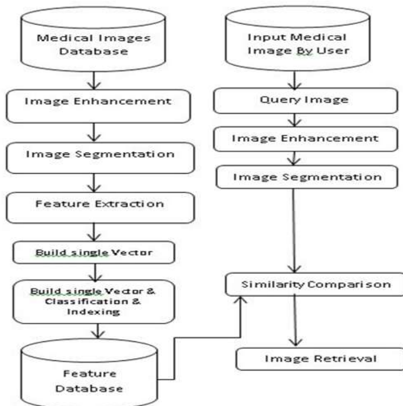
Figure1. Architecture of CBIR systems in medical
