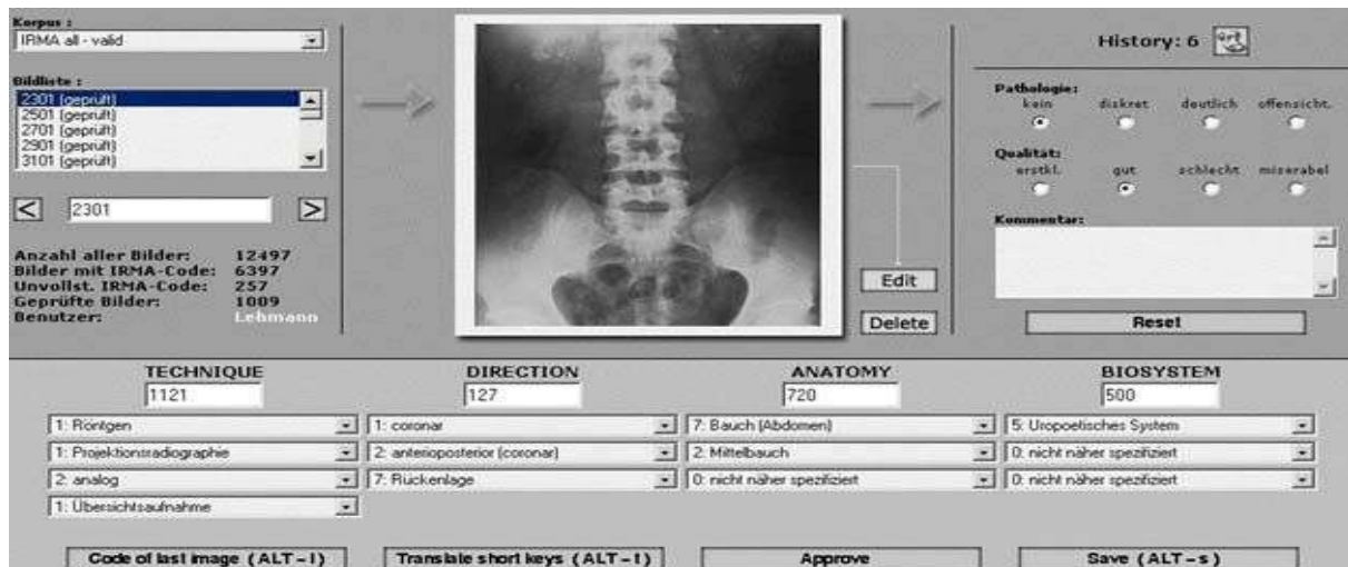
Figure 3. The IRMA image retrieval system
